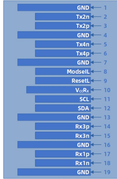
Bottom View of Board
