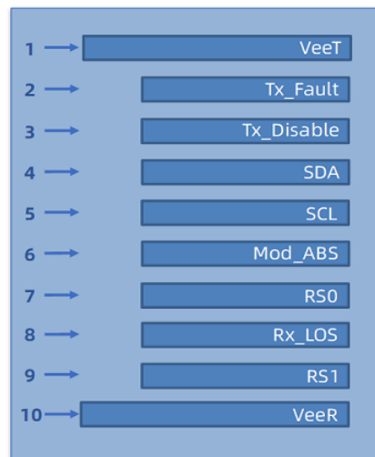
Bottom View of Board
